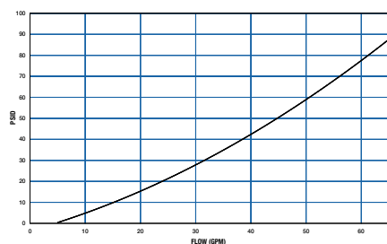
Inlet Port Thru Tank Port @ 100°F (300 SUS)
