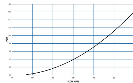
Inlet Port Thru Cooler Port @ 145°F (110 SUS)
