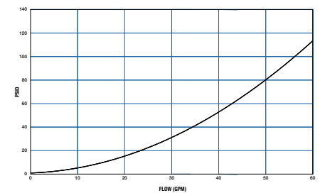
Inlet Port Over Integral Relief Valve @ 170°F (78 SUS)
